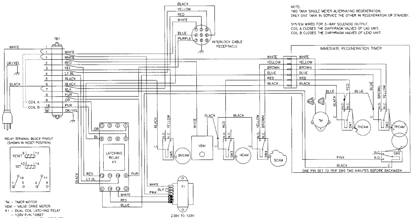
REMOTE METER WIRING
