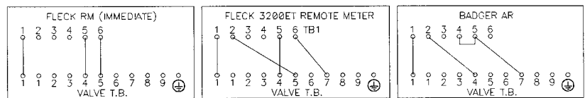
REMOTE METER WIRING
